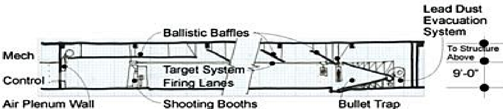
Firing Range Section
