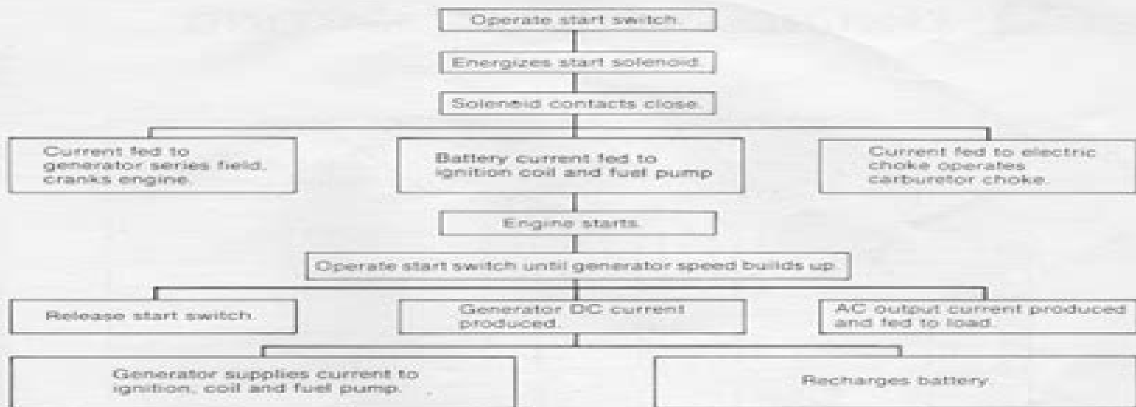
FIGURE 5. SEQUENCE OF OPERATION
