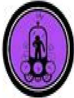
Bilker Paradox
