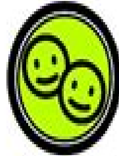
Twin Paradox
