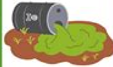
Chemical pollution
