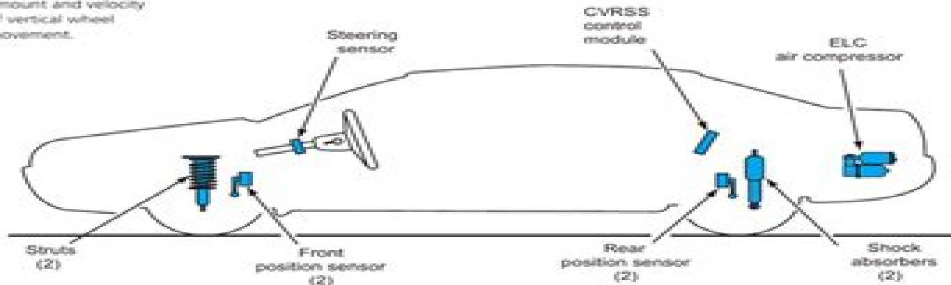
Figure 8-45 Continuously variable road sensing suspension (CVRSS) system components.
