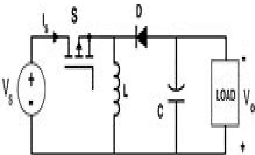
Buck-Boost Converter
