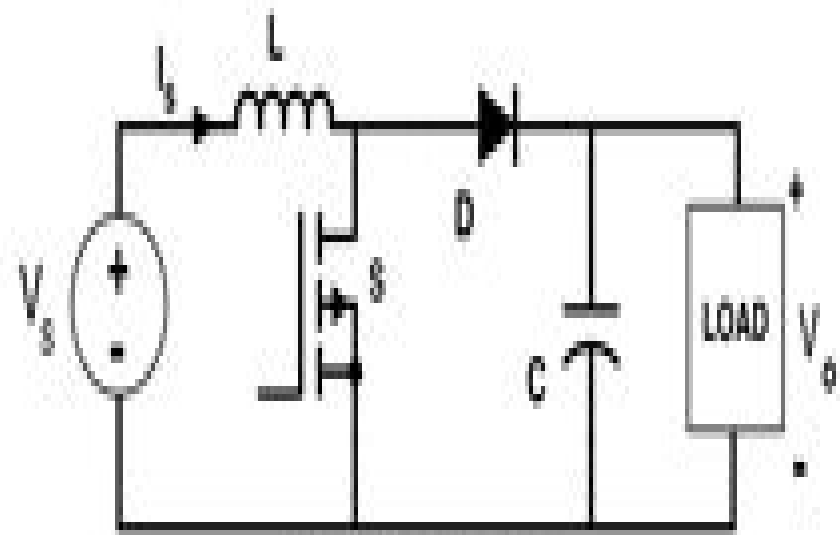
Boost Converter
