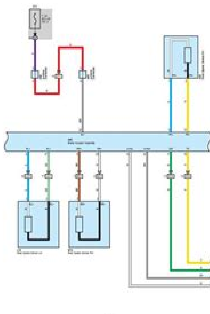
Wiring Diagram: Power Window Control, PWL, PWL
