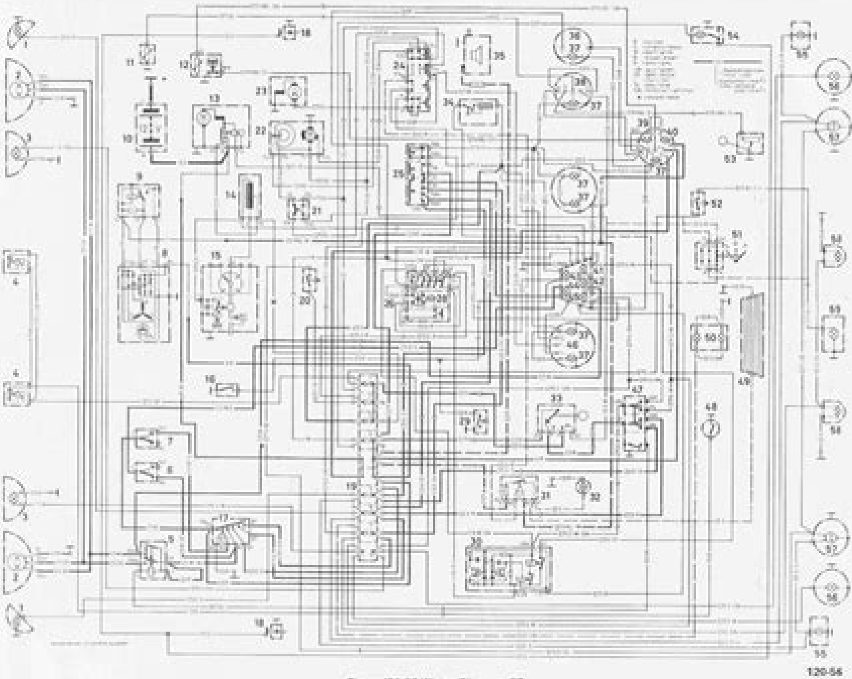
Figure 120-56 Wiring Diagram GT
